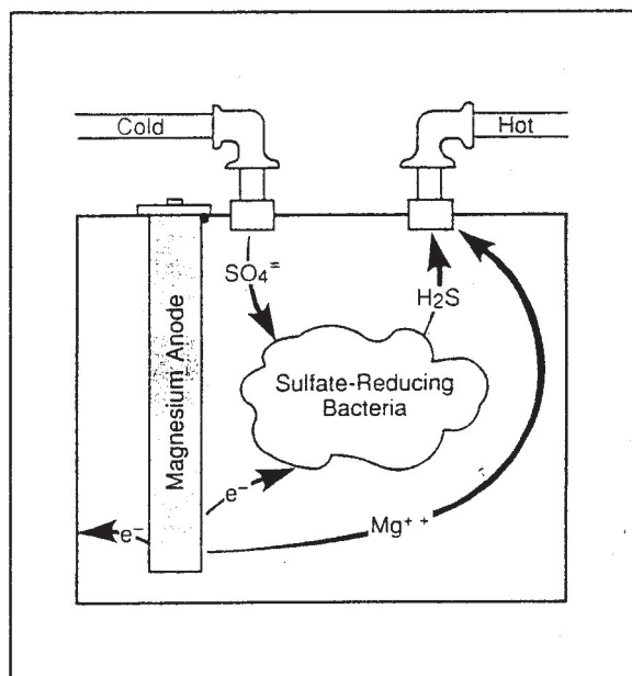
Figure 1 Bacterial action in water heater.
